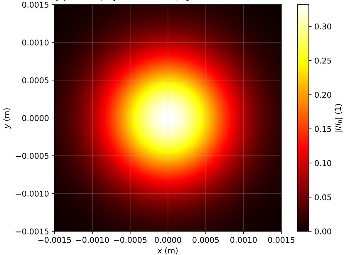
Intensity profile I(x, y, z = 3.582m)/I_0 , P_{in}=0.3P_{cr} , artificial time
